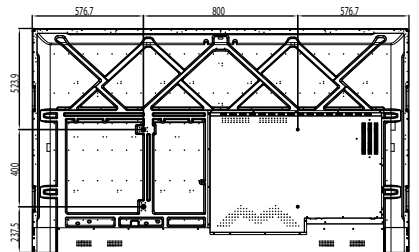
Wall Mount
